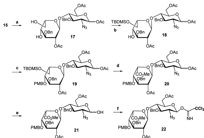
Scheme 6. Reagents and conditions: (a) 80% aq AcOH, 100°C, 1 h, 72%; (b) TBDSO, DMAP, Et 3 N, CH 2 Cl 2 , rt, 95%; (c) PMBO-C(NH)CCl 3 , TfOH, CH 2 Cl 2 -Et 2 O, rt, 2 h, 90%; (d) CrO 3 , H 2 SO 4 , acetone, then MeI, KHCO 3 , NBu 4 NI, DMF, 40%; (e) BnNH 2 , Et 2 O, rt, 74%; (f) CCl 3 CN, K 2 CO 3 , 4 Å MS, CH 2 Cl 2 , rt, 85%.
