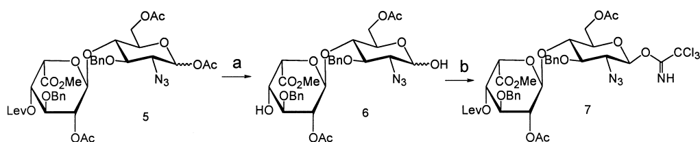
Scheme 4. Reagents and conditions: (a) \text{BnNH}_2 , \text{Et}_2\text{O} , rt, 83%, (b) \text{CCl}_3\text{CN} , \text{K}_2\text{CO}_3 , 4 Å MS, \text{CH}_2\text{Cl}_2 , rt, 81%.
