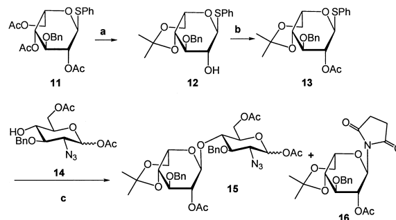
Scheme 5. Reagents and conditions: (a) MeONa, MeOH, then \text{Me}_2\text{C}(\text{OMe})_2 , CSA, rt, 84% (two steps); (b) \text{Ac}_2\text{O} , Pyr, rt, 96%; (c) NIS, TfOH, 4 Å MS, \text{CH}_2\text{Cl}_2 , 0°C, 15 (80%), 16 (10%).
