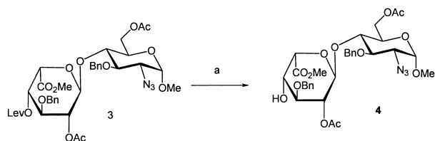
Scheme 3. Reagents and conditions: (a) \text{N}_2\text{H}_4 , AcOH, Pyr, rt, 90%.
