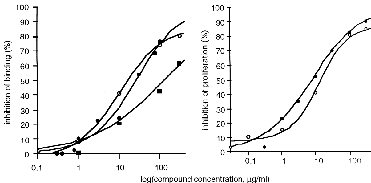
Figure 1. Effect of heparin (○), 1 (■) or 2 (●) on the binding of 125 I-FGF-2 to HASMC (left panel) and on the mitogenic effect of FGF-2 for HASMC (right panel).
